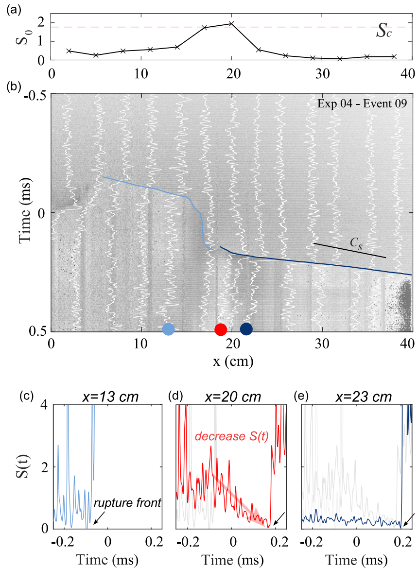
Figure 6. Representative example of barrier-induced supershear transition. (a) Initial S ratio computed along the default. The red dotted line indicates the S_c value. (b) Videogram of the selected event, with synchronized shear stress measurements (in white). Light and dark blue curves indicate the rupture front of the subshear and supershear propagation phases respectively. Markers indicate the location at which S(t) was computed. (c–e) Temporal evolution of S(t) for the three selected locations around and inside the stress barrier.
