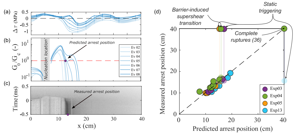
Figure 4. Rupture arrest prediction through linear elastic fracture mechanics. Detailed procedure shown for Experiment 03. (a) Non-uniform stress drop distribution for partial ruptures (Ev 02–08). (b) \frac{G_0}{G_c} distribution. The red dotted line indicates the arrest criterion for \frac{G_0}{G_c} < 1 . Complete rupture profiles are shown in Section 4.4. (c) Videogram of event 04. Purple dot marks the measured arrest; the same dot marks the predicted arrest in (b). (d) Predicted versus measured rupture arrest position for all ruptures (Exp 03,04,05,13). Partial ruptures align along the 1:1 slope, indicating good prediction, while for complete ruptures, no arrest is predicted. Shaded markers denote the location where ruptures temporarily halted before continuing to propagate further (three cases of static triggering and one case of barrier-induced supershear transition).
