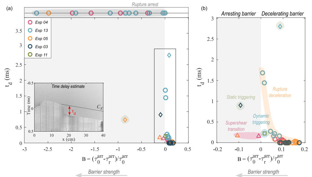
Figure 9. Time delay ( t_d ) distribution as a function of B value ( B = \frac{\tau_0^{\text{arr}} - \tau_r^{\text{arr}}}{\tau_0^{\text{arr}}} ) (a). Marker color indicates the corresponding experiment, and marker shape denotes the interaction mechanism: circles represent classical LEFM behavior (rupture arrest or deceleration), diamonds indicate static triggering, triangles indicate barrier-induced supershear transition, and squares indicate dynamic triggering. Arrested ruptures, which are not characterized by any t_d , are shown aligned above the main plot, and all fall in the B < 0 domain. The remaining events fall into the B > 0 domain, with a few exceptions, and their t_d values cover a range between 0.1 and 2.8 ms. The inset illustrates the procedure used to estimate the time delay. (b) Zoom of panel (a).
