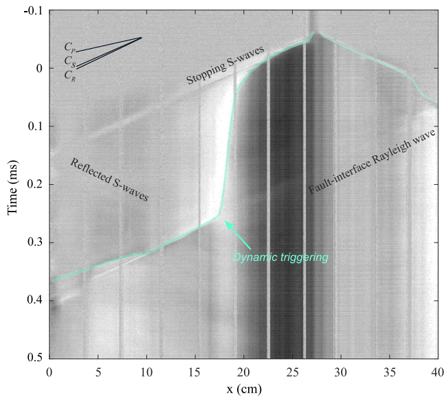
Figure 8. Videogram of the selected example of dynamic triggering. Labels indicate the generated (and/or reflected) seismic waves. The green curve highlights the rupture front.
