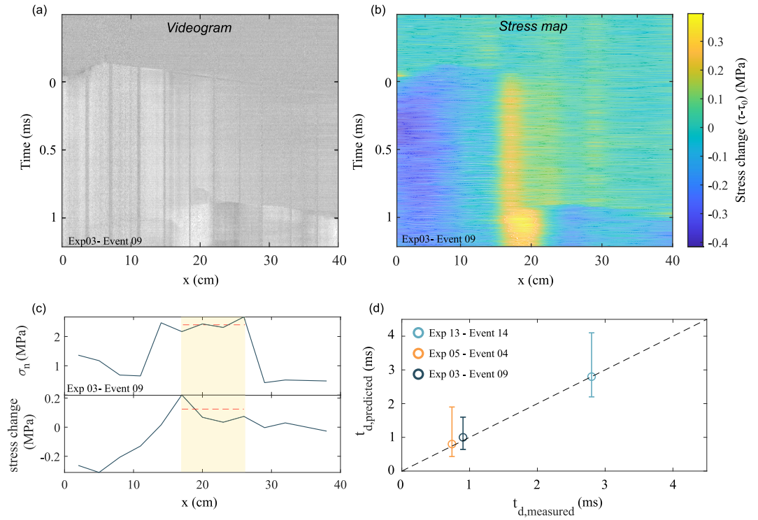
Figure 5. (a) Videogram of one representative example of static triggering (Experiment 03–Event 09). (b) Shear stress change map for the event in (a), obtained by spatially interpolating stress measurements from strain gauges. (c) Initial normal stress distribution (top) and shear stress change before triggering (bottom). The yellow shaded area indicates the area interested by stress change due to the original event. The dashed red line indicates the average value used in Equation 5. (d) Comparison between the expected delay time t_i and the measured delay time t_d for the three observed cases.
