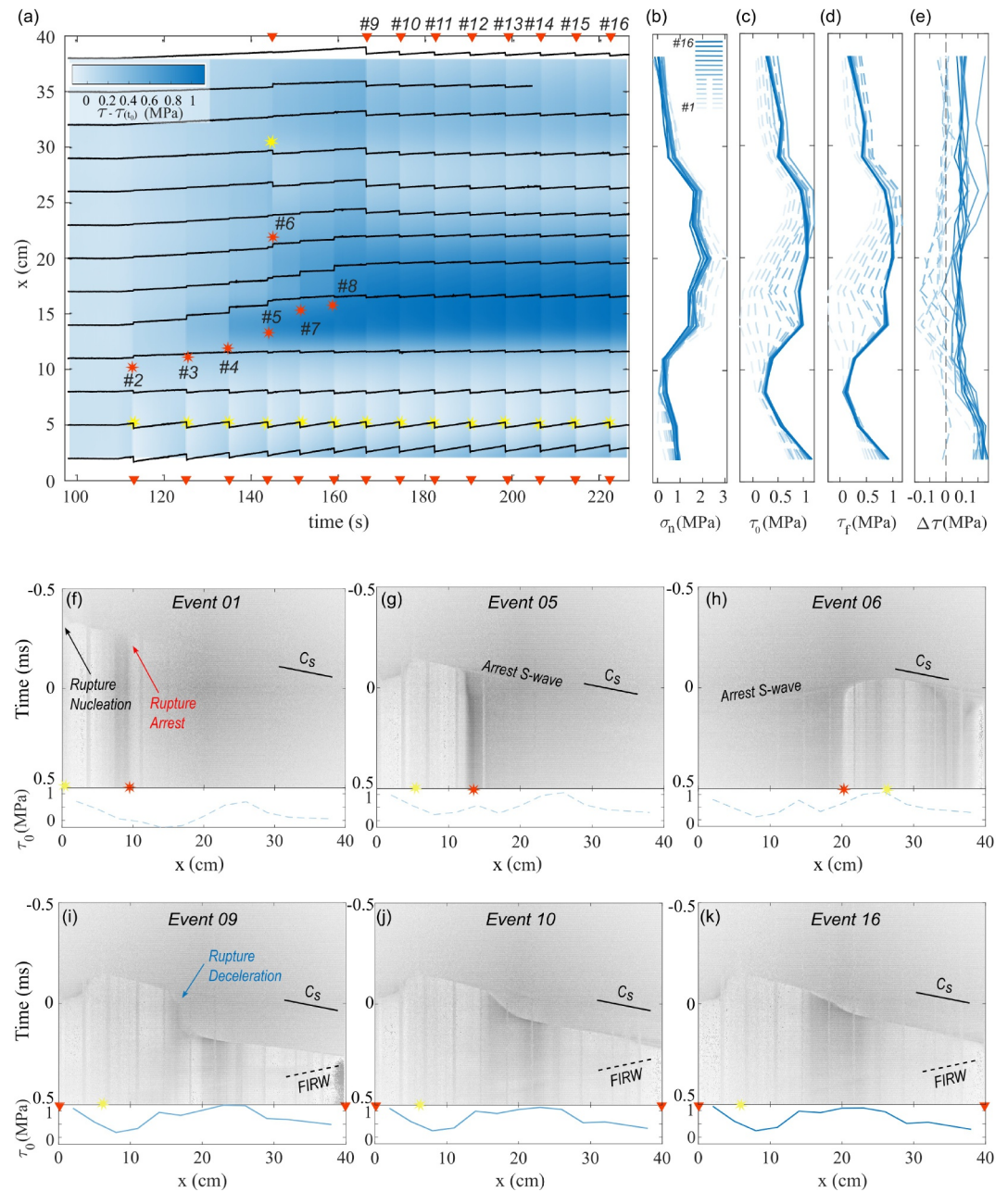
Figure 2. Results of a representative experiment (Exp 04). (a) Temporal evolution of shear stress at 13 measuring locations. The curves are offset on the y-axis by the measuring location. In the background, the shear stress distribution obtained by spatial interpolation of the mechanical measurements, with respect to the time t_0 = 100 s. For each event, a yellow star marks the nucleation location, a red star marks the arrest location, and red triangles mark ruptures that reach the free edge of the interface, as measured on the videograms. (b, c) indicate the background normal and shear stress spatial distribution before each rupture, (d) the final shear stress after each rupture, and (e) the potential stress drop ( \Delta\tau = \tau_0 - \tau_{res} ). Note that the residual stress \tau_{res} is defined as the final stress ( \tau_f ) of complete ruptures. Dashed curves refer to partial events, and solid curves to complete events. (f–m) show characteristic videograms of selected events. A panel below each subplot shows the initial shear stress before the event (similar to (c)). In particular, (f–h) show partial events, and (i–k) complete events.
