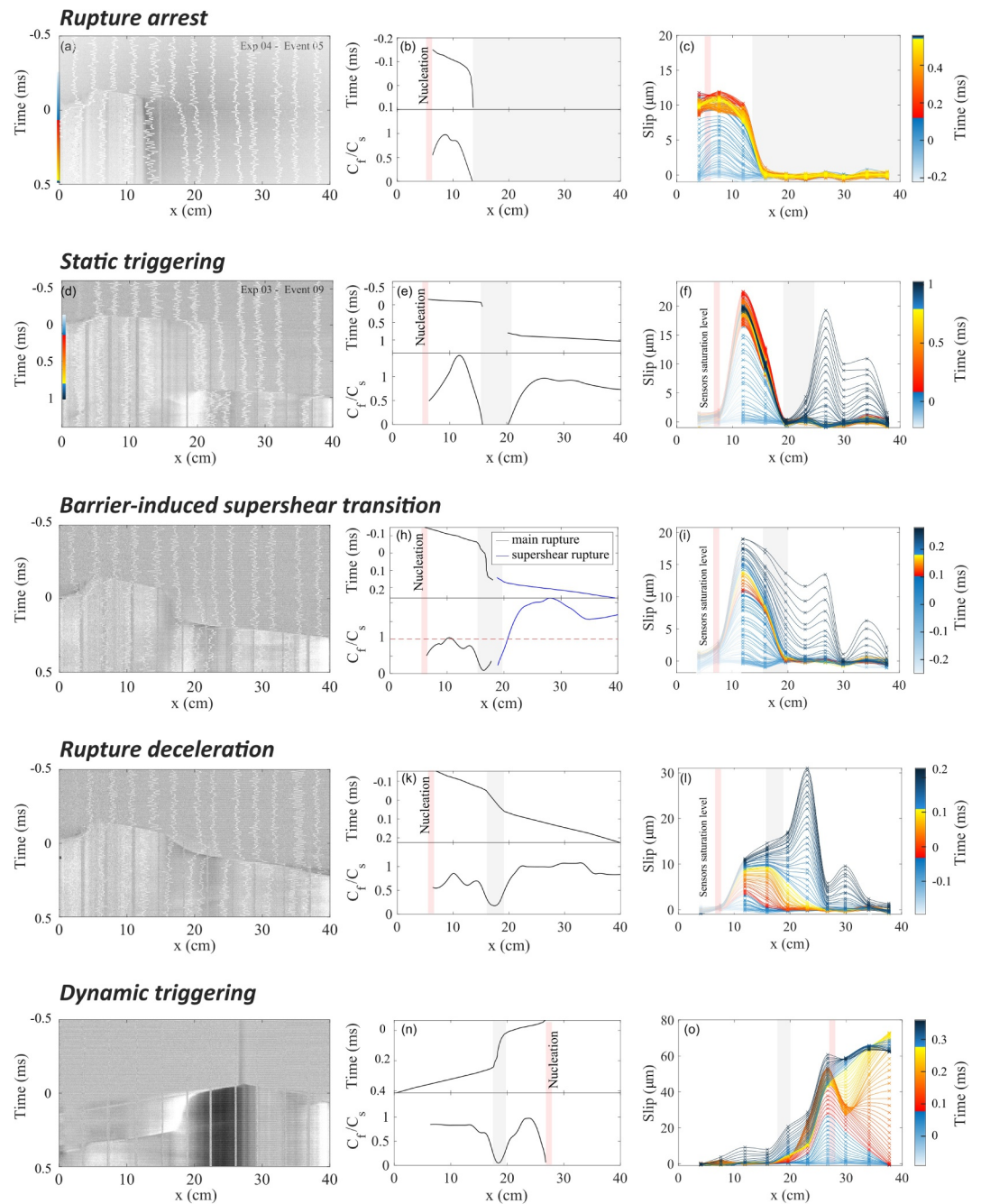
Figure 3. Collection of all representative rupture styles interacting with a stress barrier. (a, d, g, j, m) videogram of the selected rupture, with synchronized shear stress measurements (in white) obtained through the thirteen strain gauge rosettes. Colorbar on the left indicates the time interval selected for subplots (c, f, i, l, o). (b, e, h, k, n) rupture front evolution, obtained through manual picking from the videogram (on the top), and rupture propagation velocity (on the bottom). The red-shaded region indicates the rupture nucleation location, while the gray area indicates a region of either arrest (b) or deceleration (e, h, k, n). (c, f, i, l, o) Spatiotemporal slip distribution during each event. The curves are plotted with a time interval of 5 \mu s. Note that a different colormap (orange) indicates the period during rupture deceleration. A shaded area indicates cases in which the displacement sensors reached saturation, making their measurements unreliable ( x = 3\text{--}10 cm for f, i, l, o).
