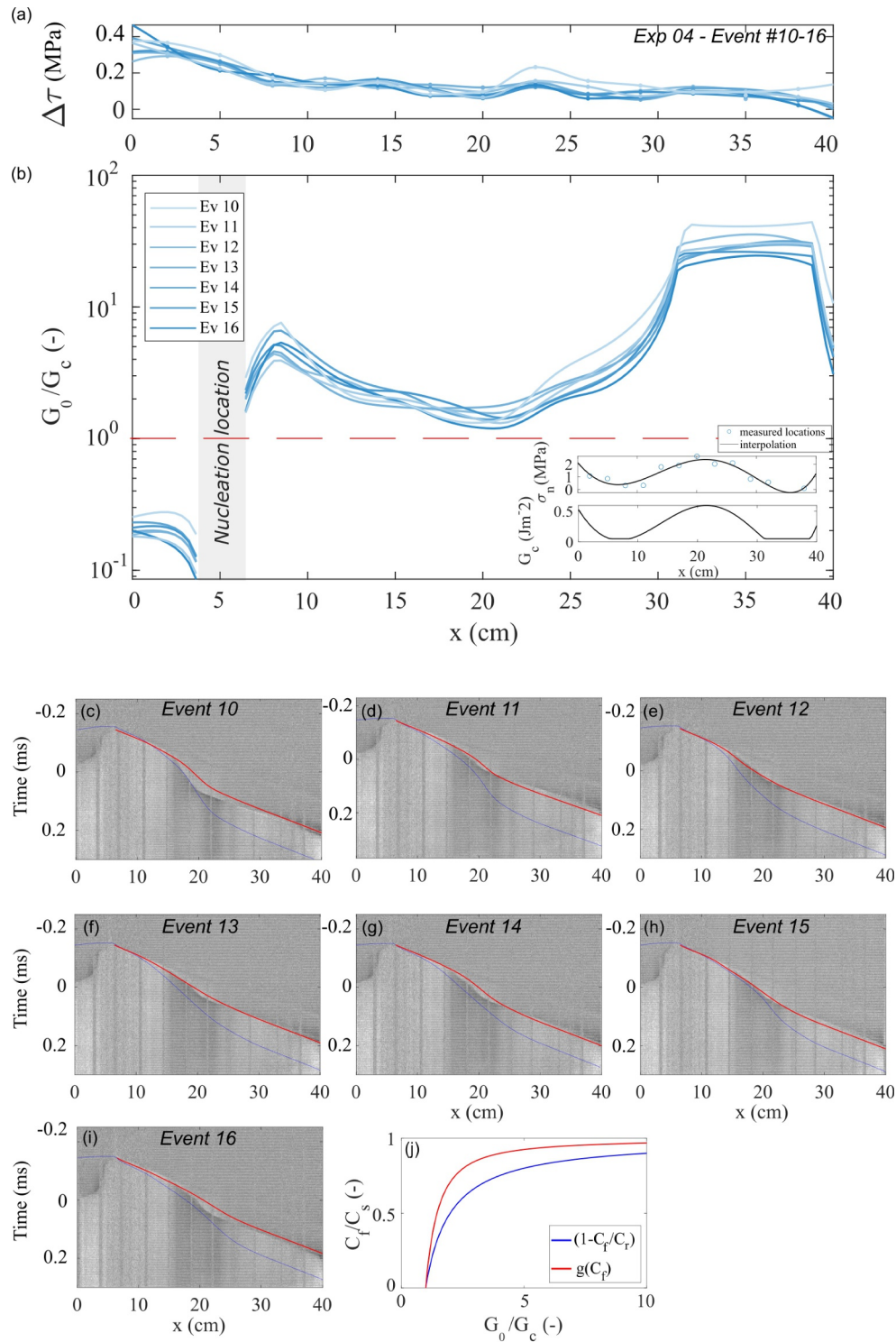
Figure 7. Rupture front prediction through LEFM for Experiment 04. (a) Non-uniform stress drop distribution for all studied partial ruptures (Ev 10–16). (b) \frac{G_0}{G_c} distribution for all ruptures. The red dotted line indicates the arrest criterion for \frac{G_0}{G_c} < 1 . The inset shows the normal stress distribution and the assumed fracture energy profile. (c–i) Videograms of Ev 10–16 with rupture front prediction using the approximated velocity function (in blue), and its exact solution (in red). (j) Approximation and exact solution for the velocity function g(C_r) as a function of rupture speed and energy ratio.
