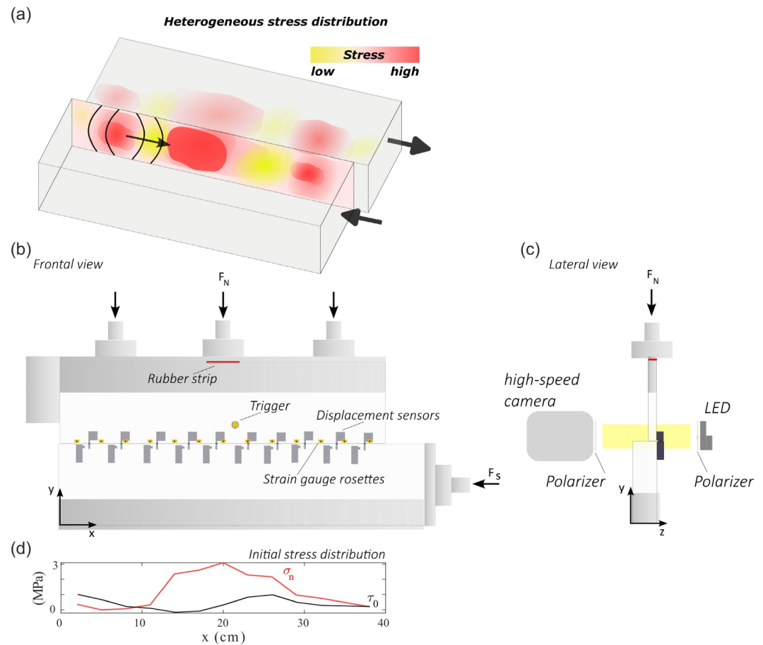
Figure 1. Experimental apparatus located at ESEILA in Geoazur, Université Côte d’Azur. (a) Sketch of the laboratory fault system, subjected to heterogeneous stress conditions. (b) Frontal view. Two PMMA samples are positioned one on top of the other to generate a 40 \times 1 cm bare interface. Thirteen strain gauge rosettes and ten displacement sensors are positioned at equidistant locations along the fault. A piezoelectric sensor glued in the middle of the fault acts as a trigger to activate camera recording. A rubber strip located below the central piston modifies the externally applied stress. (c) Lateral view reveals the presence of a high-speed camera positioned exactly in front of the artificial fault. On the opposite side, a white light is emitted and polarized for the first time. After being transmitted through the sample, it is polarized once again (perpendicularly to the direction of the first polarization), before reaching the camera lens. (d) Normal and shear stress distribution at the beginning of a representative experiment.
