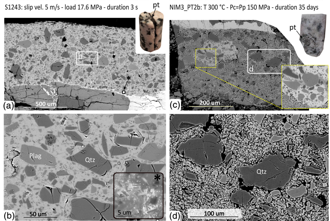
Figure 2. Pseudotachylite alteration in experiments. (a, b) Fresh experimental pseudotachylite vein; see the up-right inset in (a) for a macroscopic view of the sample. Pseudotachylite produced through a high-velocity rotary shear experiment with SHIVA starting from a tonalite from the Adamello batholith (host rock of the Gole Larghe Fault Zone). The experimental pseudotachylite vein consists of quartz and plagioclase clasts immersed into a glassy to cryptocrystalline matrix with andesitic composition (see Figure S5) and a negligible amount of porosity in the form of cooling microcracks (BSE-SEM images). Embayed quartz and plagioclase clasts (also with cusped-lobate borders) indicate progressive melting, while biotite is almost absent as clast due to selective melting (b). Locally, few micrometers in size plagioclase microlites crystallized from the melt (inset in b). (c, d) Experimental pseudotachylite (a, b) after long term (35 days) hydrothermal test ( P_c = P_p = 150 MPa, T = 300^\circ\text{C} ). The up-right inset in (c) shows that the altered pseudotachylite turned into a grayish layers macroscopically different from the original black one. The altered pseudotachylite vein consists of a clastic layer characterized by a striking increase of porosity with respect to the original one in panel (a). Quartz and plagioclase clasts are subrounded and are immersed in a microgranular matrix (c, d) (BSE-SEM images). Relics of fresh pseudotachylite are still preserved (see down-right inset with yellow border in panel c) and allowed to track the evolution of the alteration process. Incipient alteration produced peculiar dark porous halos which resemble the ones observed in the altered pseudotachylites of the Gole Larghe Fault Zone.
