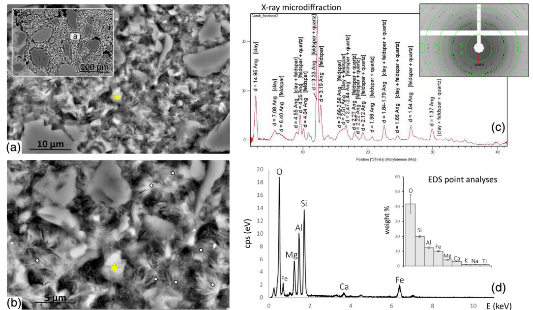
Figure 4. Advanced pseudotachylyte alteration and secondary phase nucleation. (a, b) Detail of the microporous matrix within the areas affected by more intense dissolution after hydrothermal alteration. See inset in (a) for the location of images (a) and (b). The microporous matrix consists of micrometer to submicrometer quartz and plagioclase rounded clasts and stacks of a new platy mineral phase. (c) X-ray microdiffraction has been performed on a 100 µm in size fragment of altered pseudotachylyte matrix. The resulting diffractogram is shown in (c) and was interpreted by cross-checking diffraction data with elemental EDS analyses (see d). The diffraction analysis reveals the occurrence of a smectite clay. The characteristic peak of this phase is at d = 14,85 \text{ \AA} (positioned at 2\theta = 2.71^\circ ) and is not associated to single diffraction spots (as it is the case for all the other peaks dominated by the occurrence of quartz and feldspar clasts in the analyzed fragment), but to diffraction rings, thus suggesting the polycrystalline nature of this newly formed phase. (d) Elemental EDS spot analyses of the neo-formed smectite. The selected spectrum is a representative one of the seven spot analyses performed on the sample (white circles in (b) whose elemental composition (weight % of each element) is summarized in the histogram in (d). The joined diffraction and elemental analyses suggest that the new phase is a (Ca and Mg) smectite with estimated crystallite size d = 19 \text{ nm} (see Text S4 for more details).
